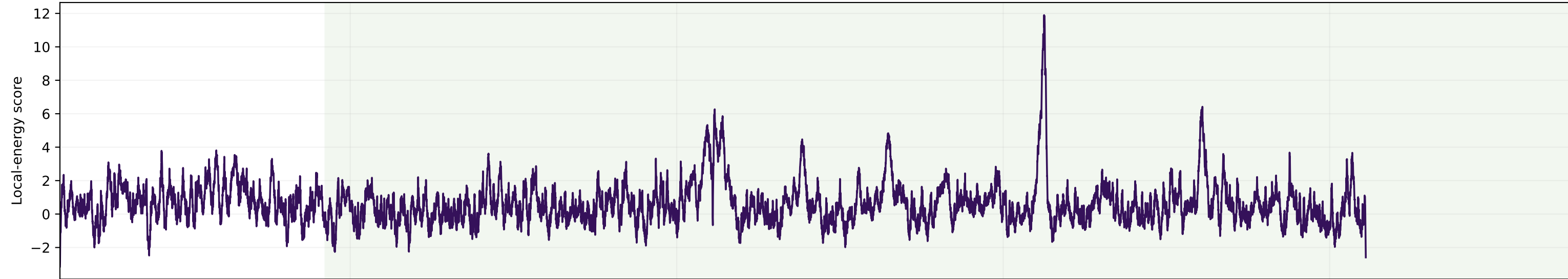
A. Cape Leeuwin H01W — 1,930 km; central travel 21.45 min
