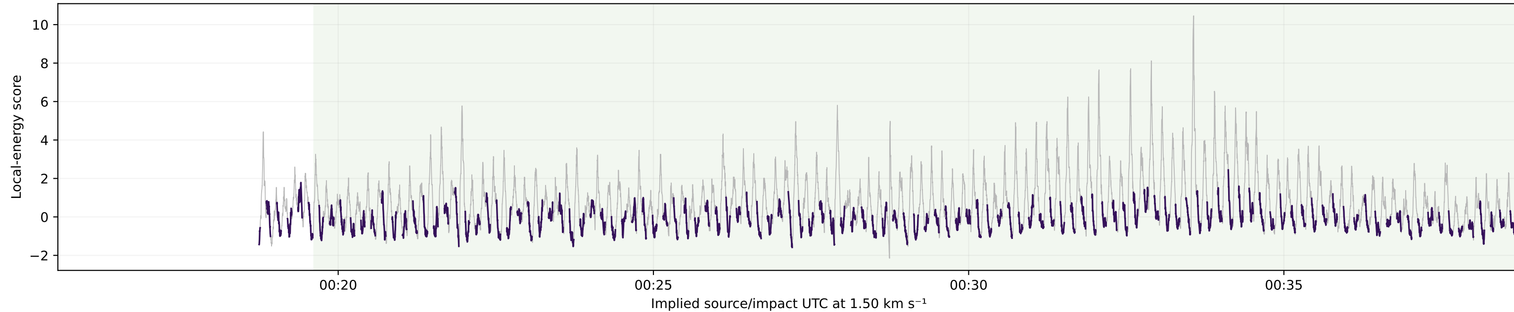
B. Diego Garcia H08S — 3,713 km; central travel 41.25 min; rank-20 residual with \pm 3 s score gaps
